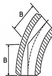
对焊45° 3D弯头 BW45° 3D Elbow
